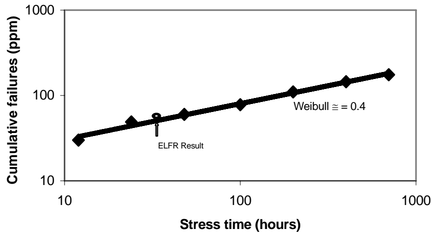
Figure 5.2 — Cumulative failures versus stress time
